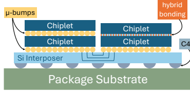
Fig. 3: 3.5D integration.
