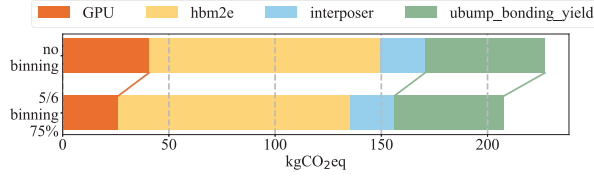
Fig. 14: NVIDIA A100 embodied carbon breakdown.
